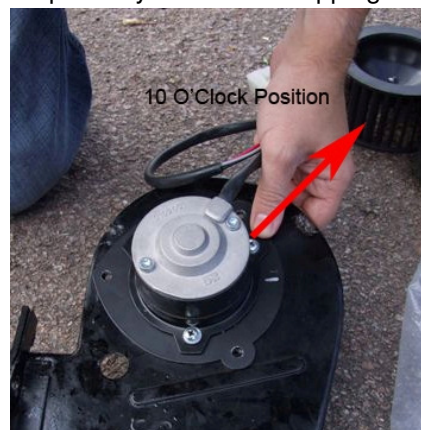
Moving Motor
